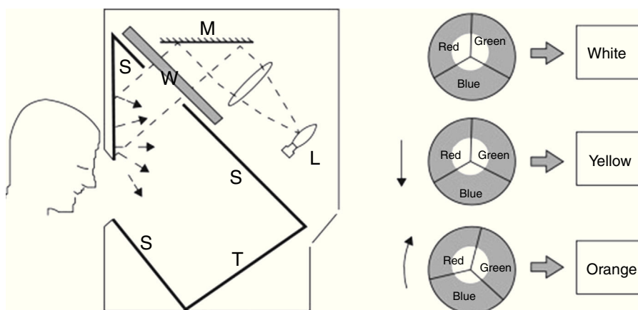
Figure 1 Cross-sectional view of the Intuitive Colorimeter. A beam of white light from a tungsten halogen lamp (L) is reflected from a mirror (M) and passes through a wheel (W) and into a box with matte white inner surfaces (S). The wheel is divided into three sectors, each covered with a different filter so as to transmit light of a different color (red, green, or blue). The colored light is mixed as it is reflected and scattered from the inner surfaces of the box. Calibrated text (T) is mounted on one surface of this box and viewed through a window in the front. Viewing distance is approximately 40 cm (2.5D). Saturation increases with eccentricity of the white beam, whereas hue changes with rotation.
