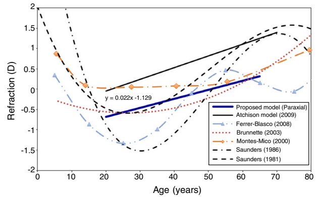
Figure 5 Variation in objective refraction with age for the unaccommodated eye. Full blue line represents linear regression fit (equation shown in graph) of the proposed model. Several clinical studies are shown for comparison.
